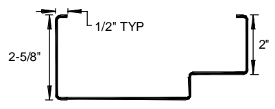
HEAD DETAIL
