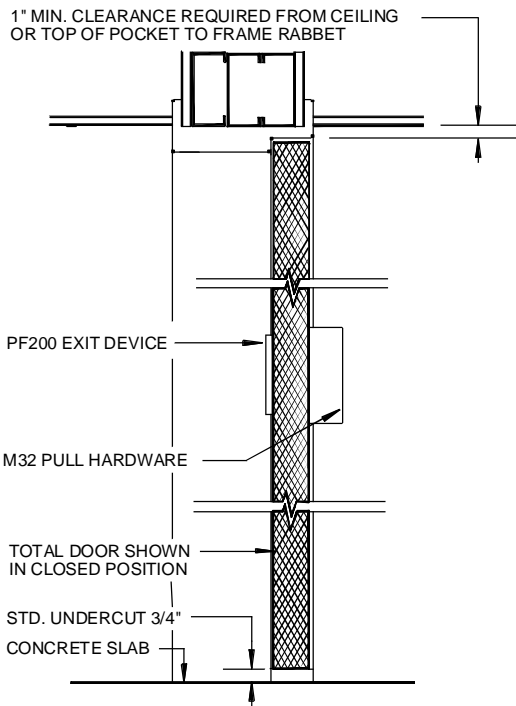
1 VERTICAL SECTION NOT TO SCALE
