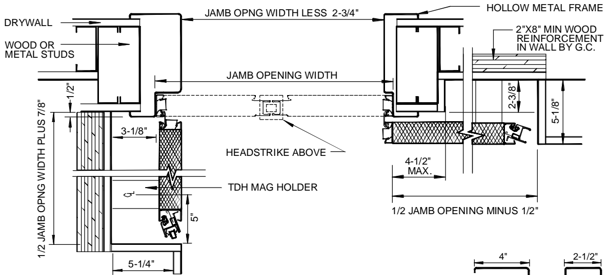
2 HORIZONTAL SECTION
