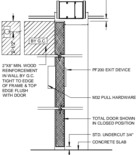
1 VERTICAL SECTION
