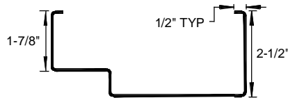
HEAD DETAIL
